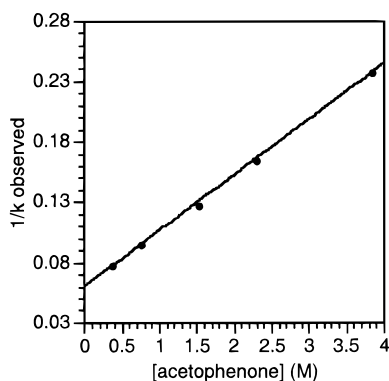
Figure 1. Plot of 1/k_{\text{obs}} (\times 10^{-4}) vs acetophenone concentration for the hydrosilation of acetophenone with \text{Ph}_3\text{SiH} .
