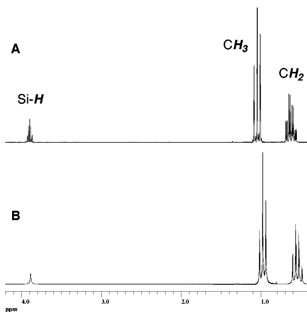
Figure 2. 300 MHz 1 H NMR spectra (C 6 D 6 , room temperature) of (A) Et 3 SiH and (B) Et 3 SiH plus 10% B(C 6 F 5 ) 3 (10 min of mixing).
